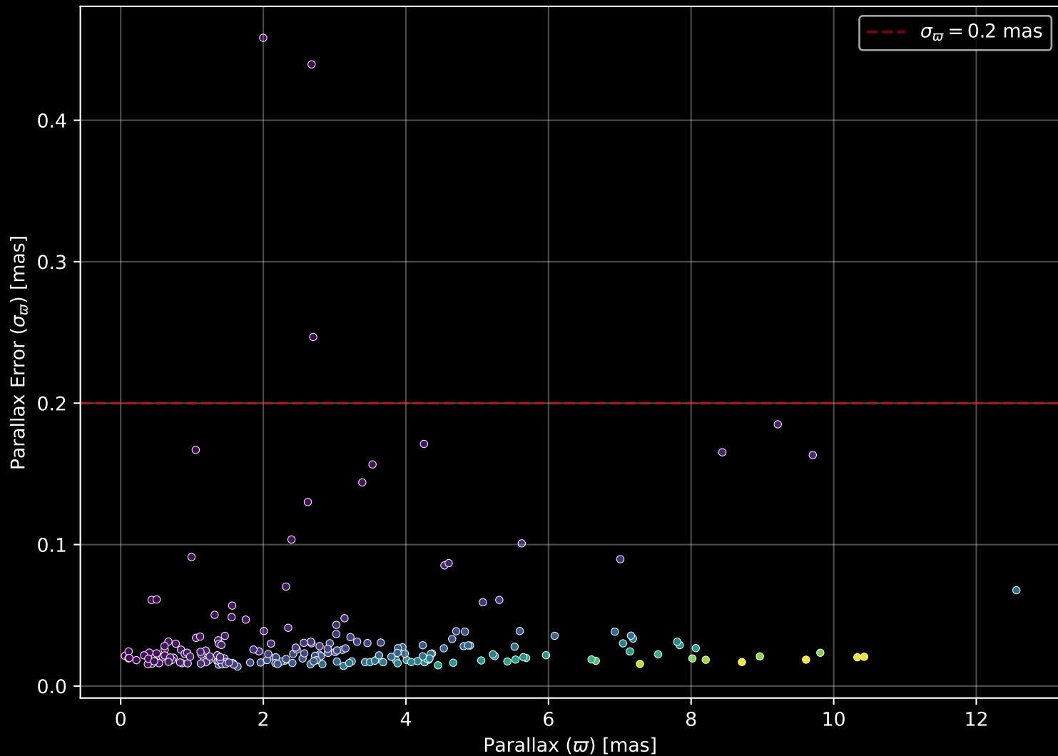
APOGEE DR17 Field: [191+44_MGA] Parallax Quality (n= 202)
