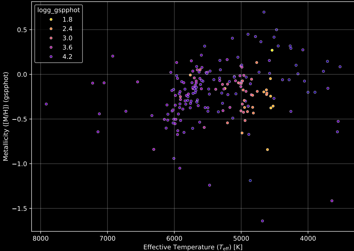
APOGEE DR17 Field: [191+44_MGA] Stellar Population Parameters (n= 202)
