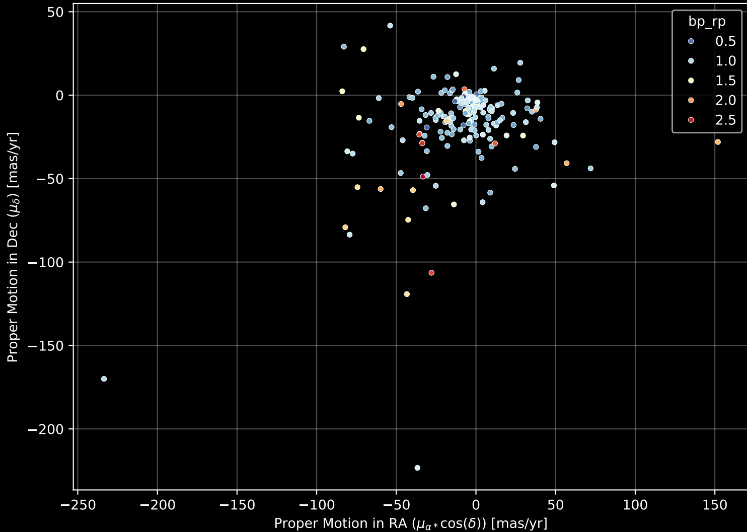
APOGEE DR17 Field: [191+44_MGA] Proper Motion Diagram (n= 202)
