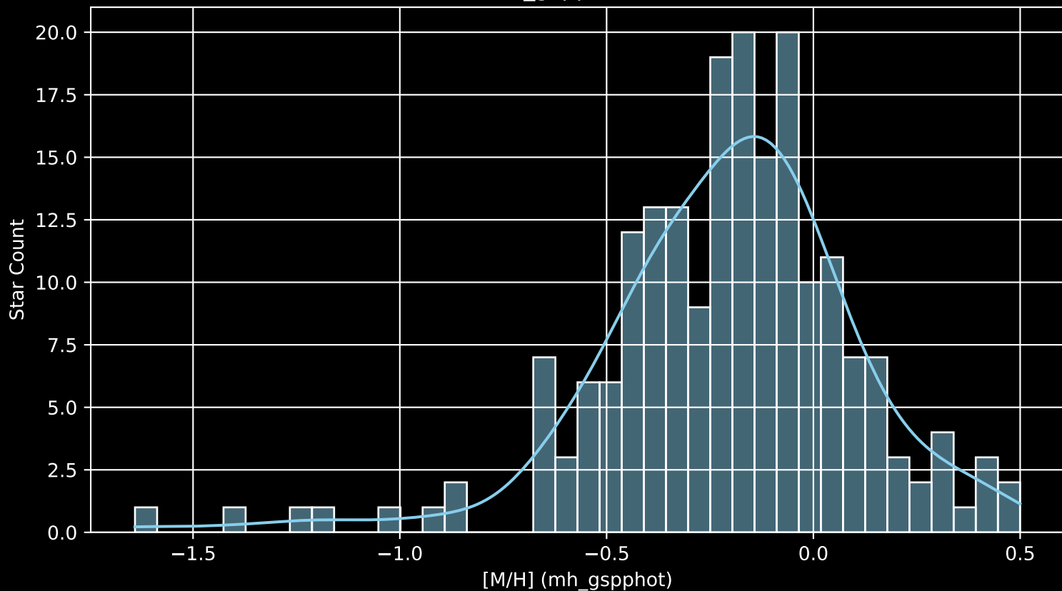
APOGEE DR17 Field: [191+44_MGA [M/H] (mh_gspphot) (n= 201)
