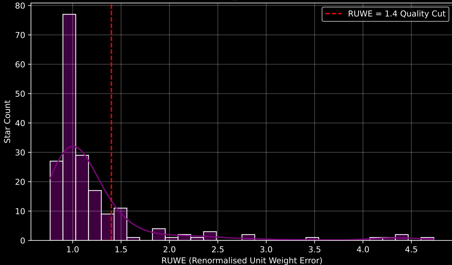
GAPOGEE DR17 Field [191+44_MGA] RUWE Distribution (n= 190)
