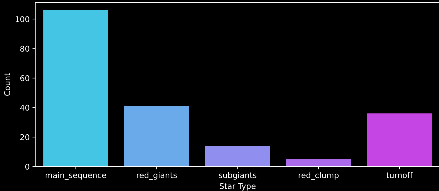
APOGEE DR17 Field: [191+44_MGA] Count plot of Star Type
